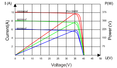
Current-Voltage&Power-Voltage Curve(360W)
