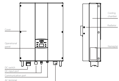
AS-IC01-(8000-10000)-2
